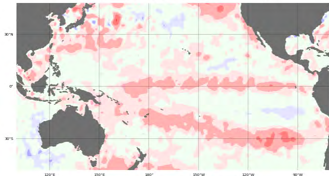
Sea surface temperature anomaly: 26/11/2018 to 02/12/2018
