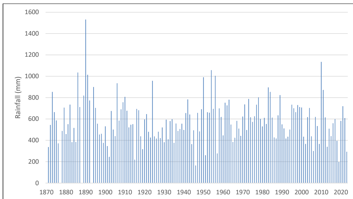
Figure 2 Annual rainfall at Roma, 1871-2023 (BOM 2024)
